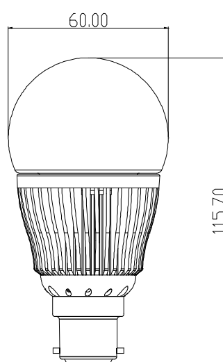
Fig 2. B22 LED Bulb Side View
