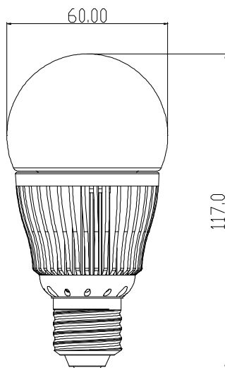
Fig 1. E27 LED Bulb Side View
